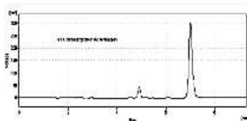
Figure 3: HPLC chromatogram of the formulation
