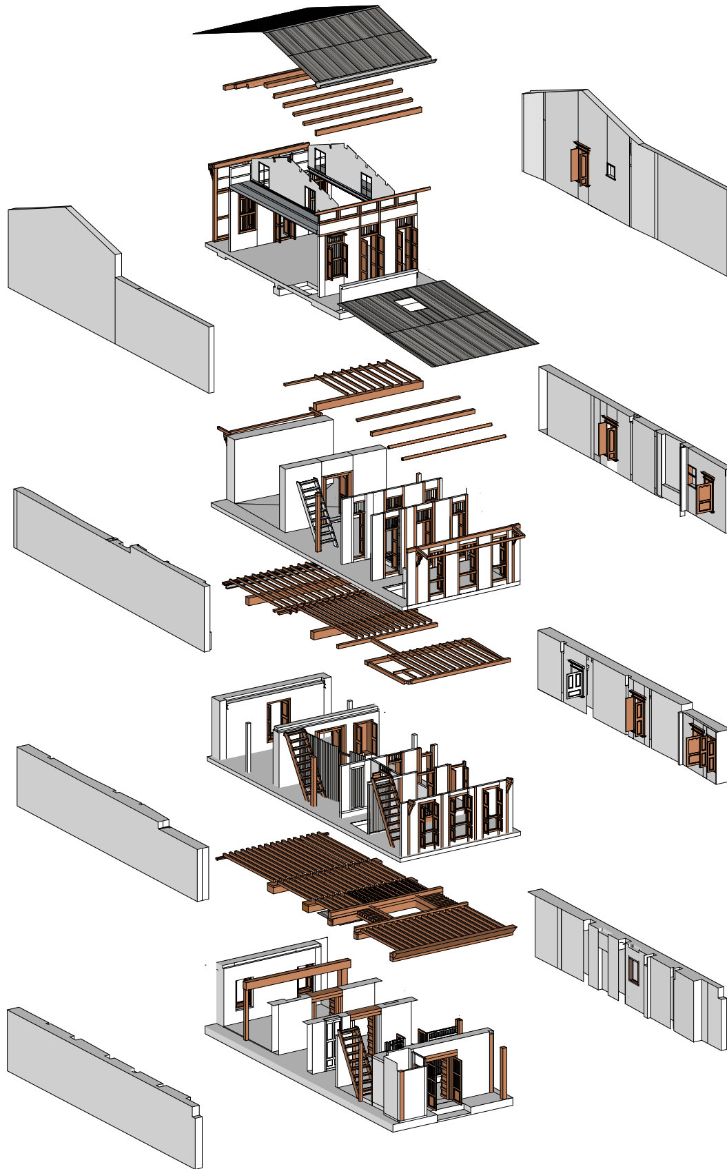
Exploded Isometric
