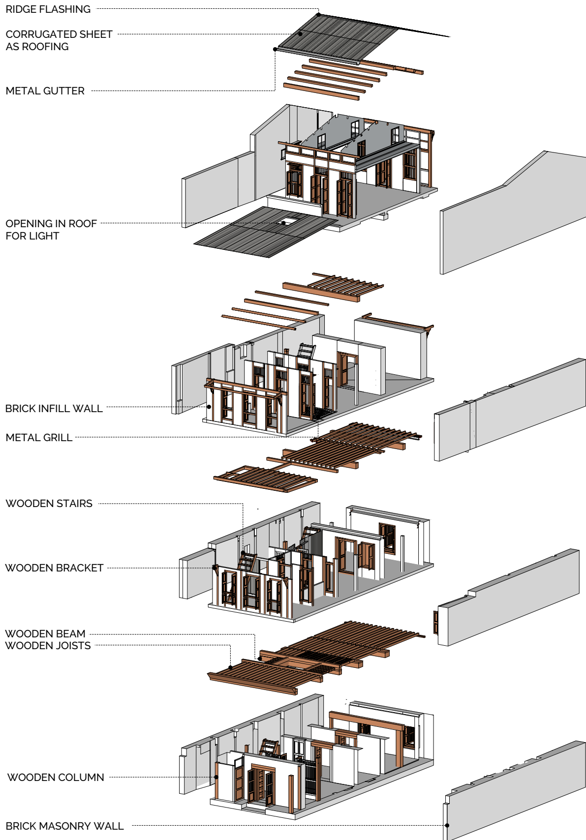
Exploded Isometric
